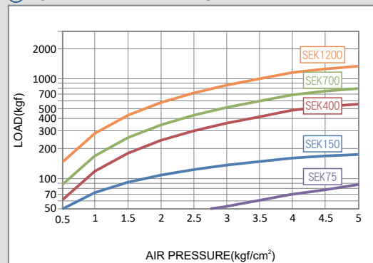
◎LOAD vs AIR PRESSURE
